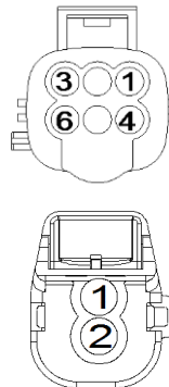
All diagrams are wire insertion view
