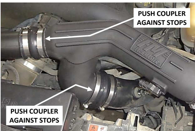
20. Push the other two couplers up against the stops on the turbo ducts and tighten the turbo duct clamps. Center the intake tube between all three couplers, so that about the same length of tube is inserted in each coupler. Then tighten the three screw clamps on the intake tube.
