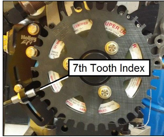
Figure 6: Aligning 7 th tooth index mark for mounting.
